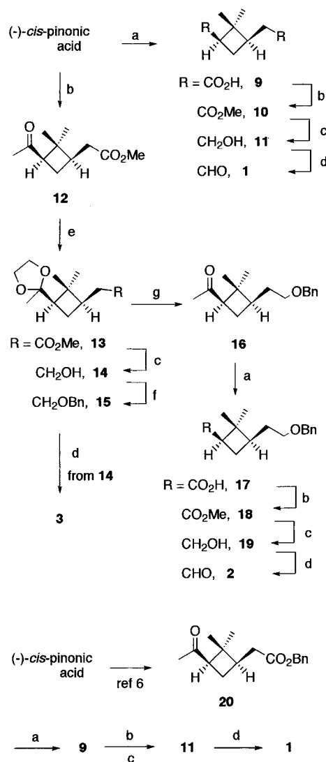
Scheme 2 a
